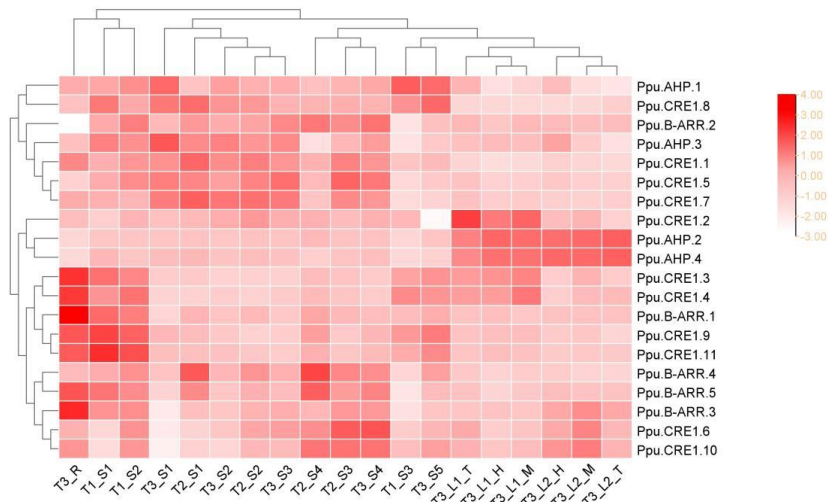
Figure 3-4 Expression analysis of elephant grass genes in each tissue
