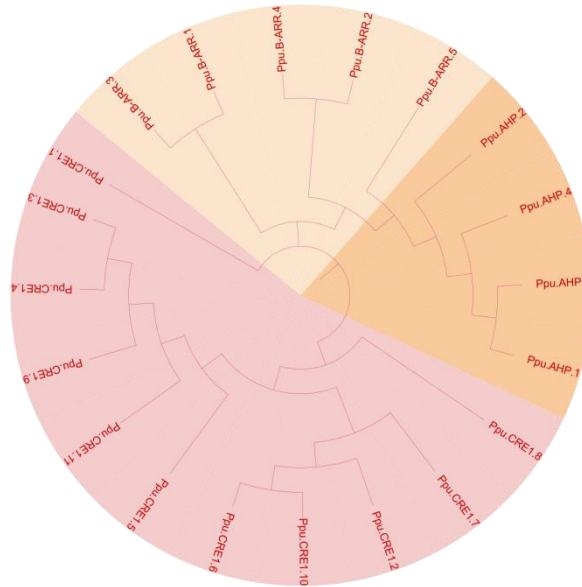
Figure 3-2 Phylogenetic analysis of 20 protein sequences in elephant grass
