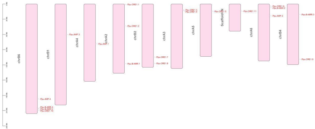
Figure 3-1 Localization of family genes on chromosomes
