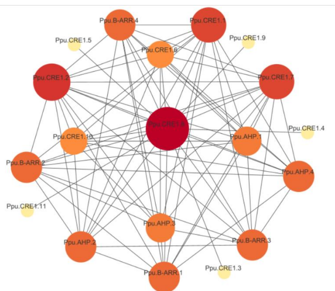
Figure 3-5 Protein interactions among the genes of the elephant grass family
