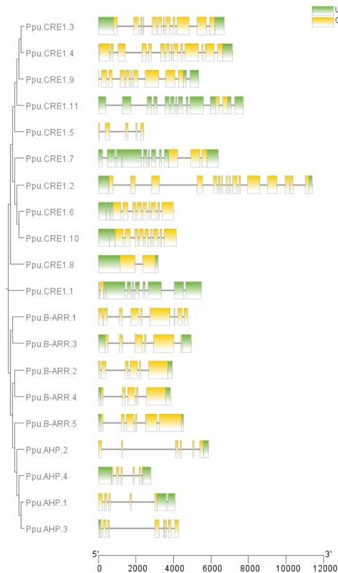
Figure 3-6 View of gene structure
